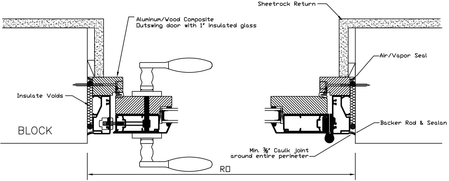
JAMB VIEW
