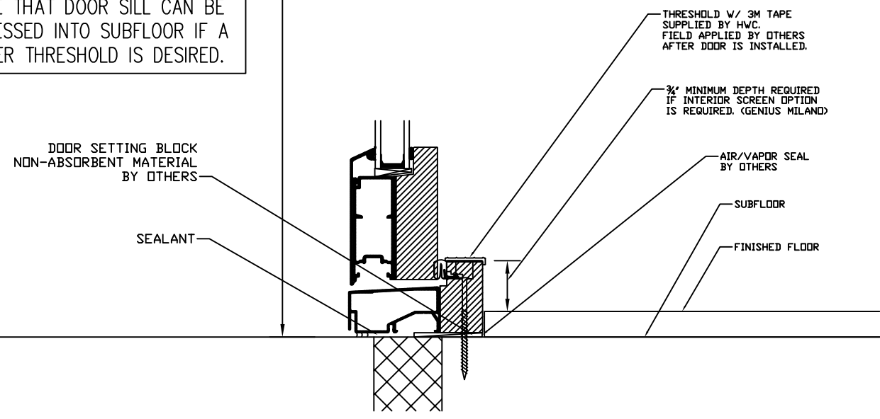
HEAD & SILL VIEW
