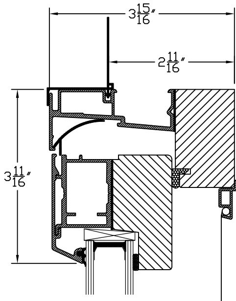
C3-1 H Head Detail Butt Hinged Casement
