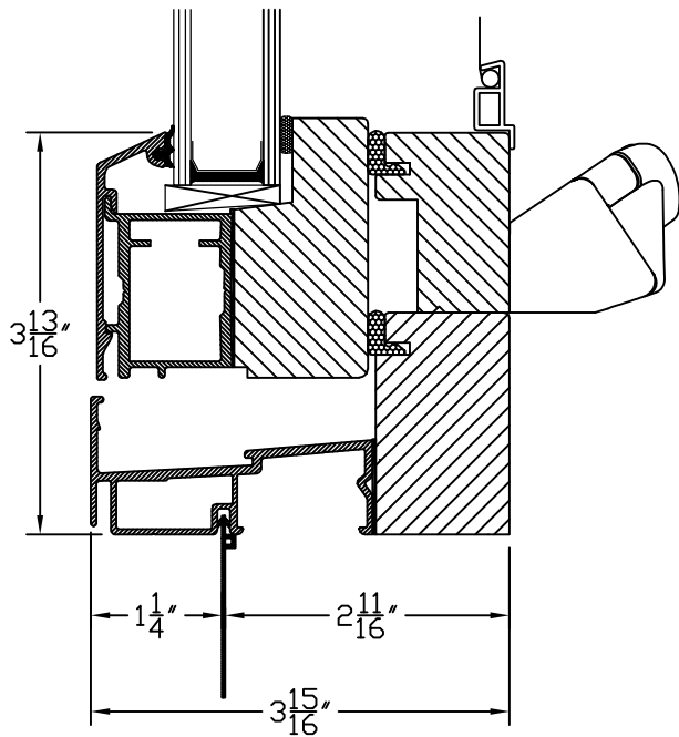
C3-3 S Sill Detail Butt Hinged Casement
