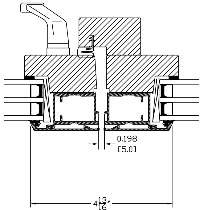
(C1-4) French Push Out Casement J Butt Hinged, Euro Handle
