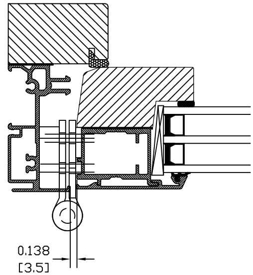
(C1-2) Jamb Detail J French Push Out Casement
