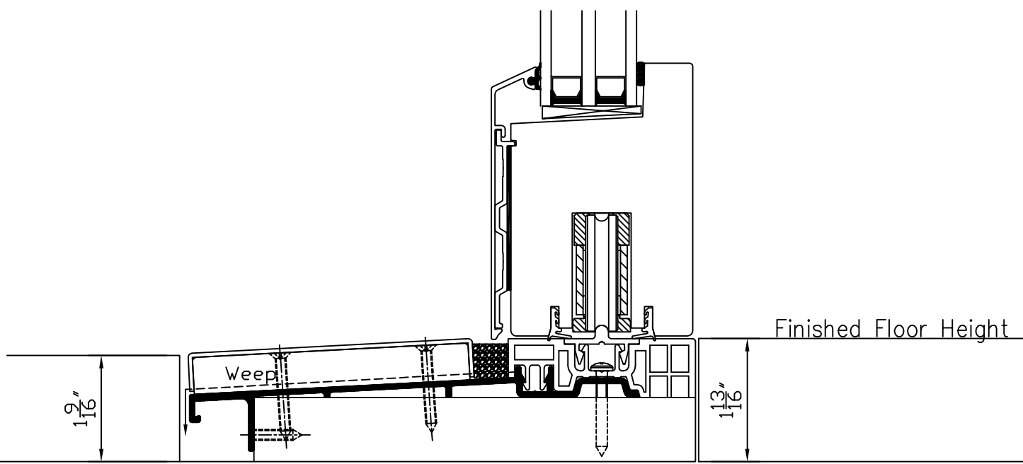
H Window Lift and Slide Head and Sill Details
