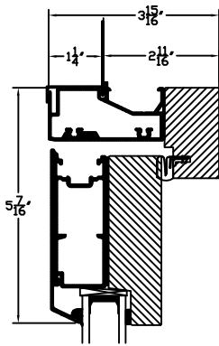
01-1 HE NORDIC OUTSWING DOOR HEAD DETAIL
