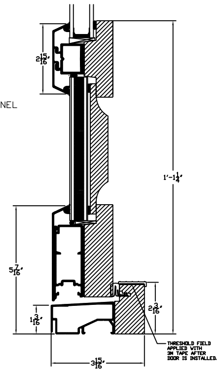
01-2 S NORDIC OUTSWING DOOR SILL DETAIL, STD KICKPANEL
