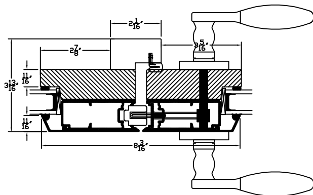
01-5 A NORDIC OUTSWING DOOR DOUBLE DOOR ASTRAGAL
