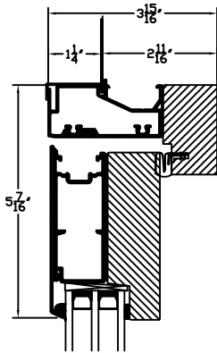
01-1 HE NORDIC OUTSWING DOOR HEAD DETAIL
