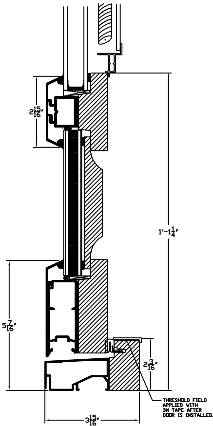
01-2 S NORDIC OUTSWING DOOR SILL DETAIL, STD KICKPANEL
