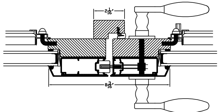
01-5 A NORDIC OUTSWING DOOR DOUBLE DOOR ASTRAGAL
