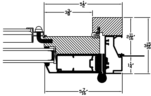
01-3 HI NORDIC OUTSWING DOOR HINGE DETAIL
